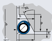
3 faces assembly HN140/240
